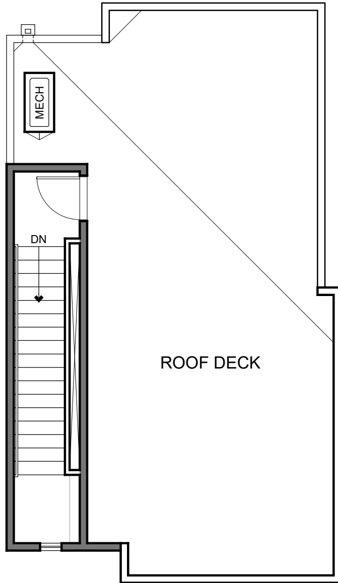
TYPE A3 ROOF DECK PLAN
